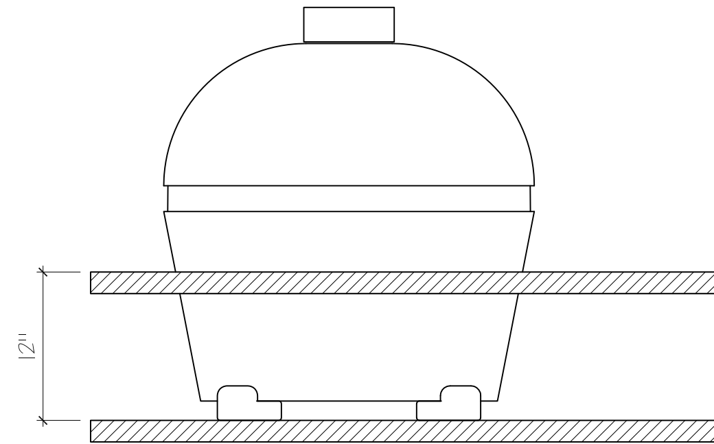
FIG. B - ELEVATION - HT. FROM TOP SURFACE TO SUPPORTING SHELF
